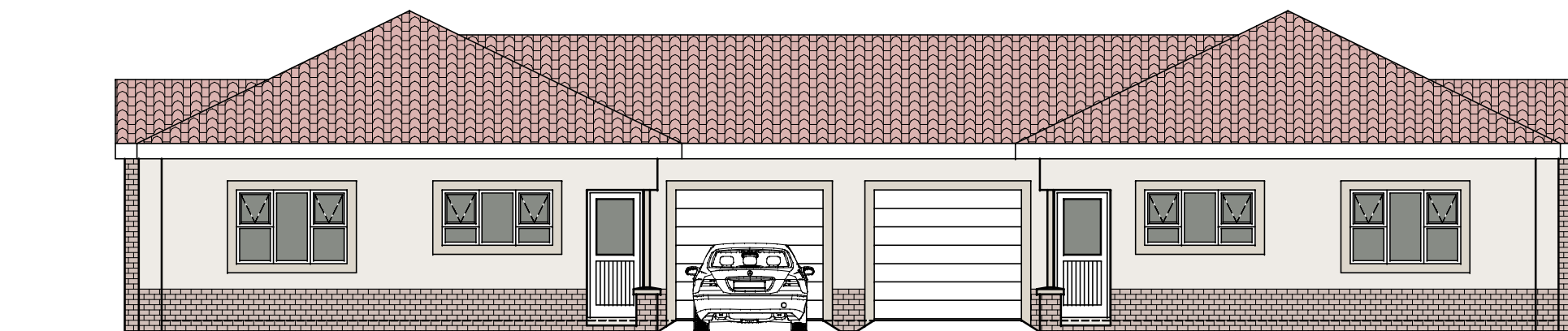
Front elevation 1:100
