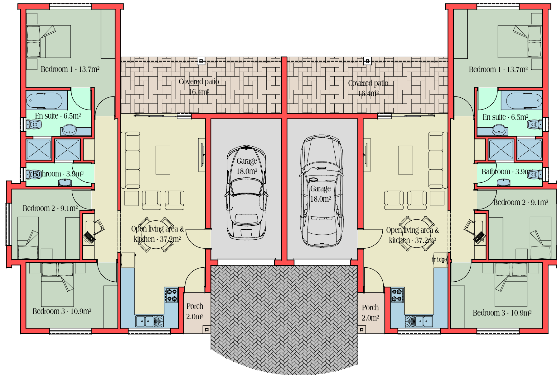
Floor plan 1:100
