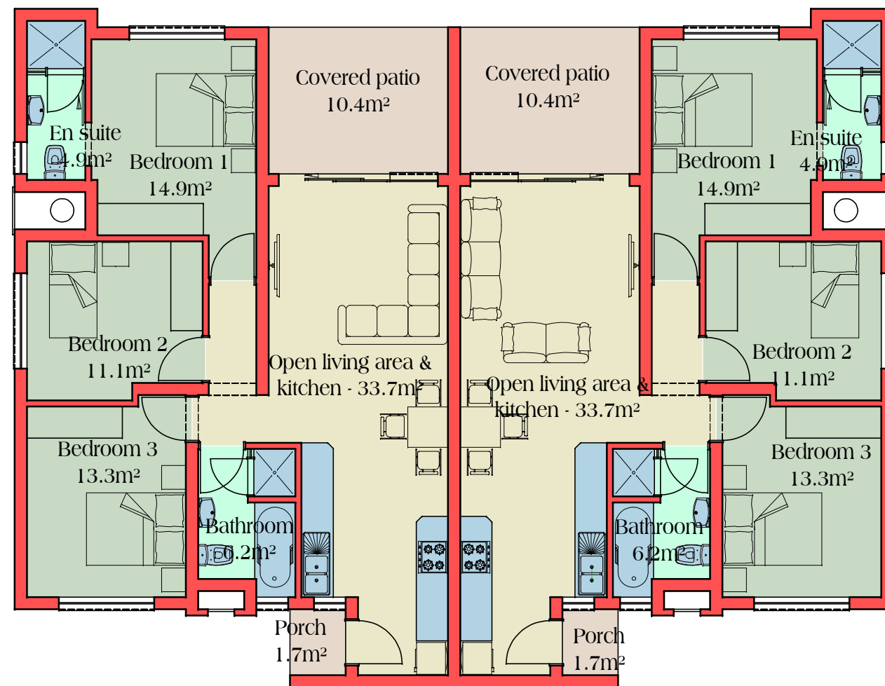
Ground floorplan
