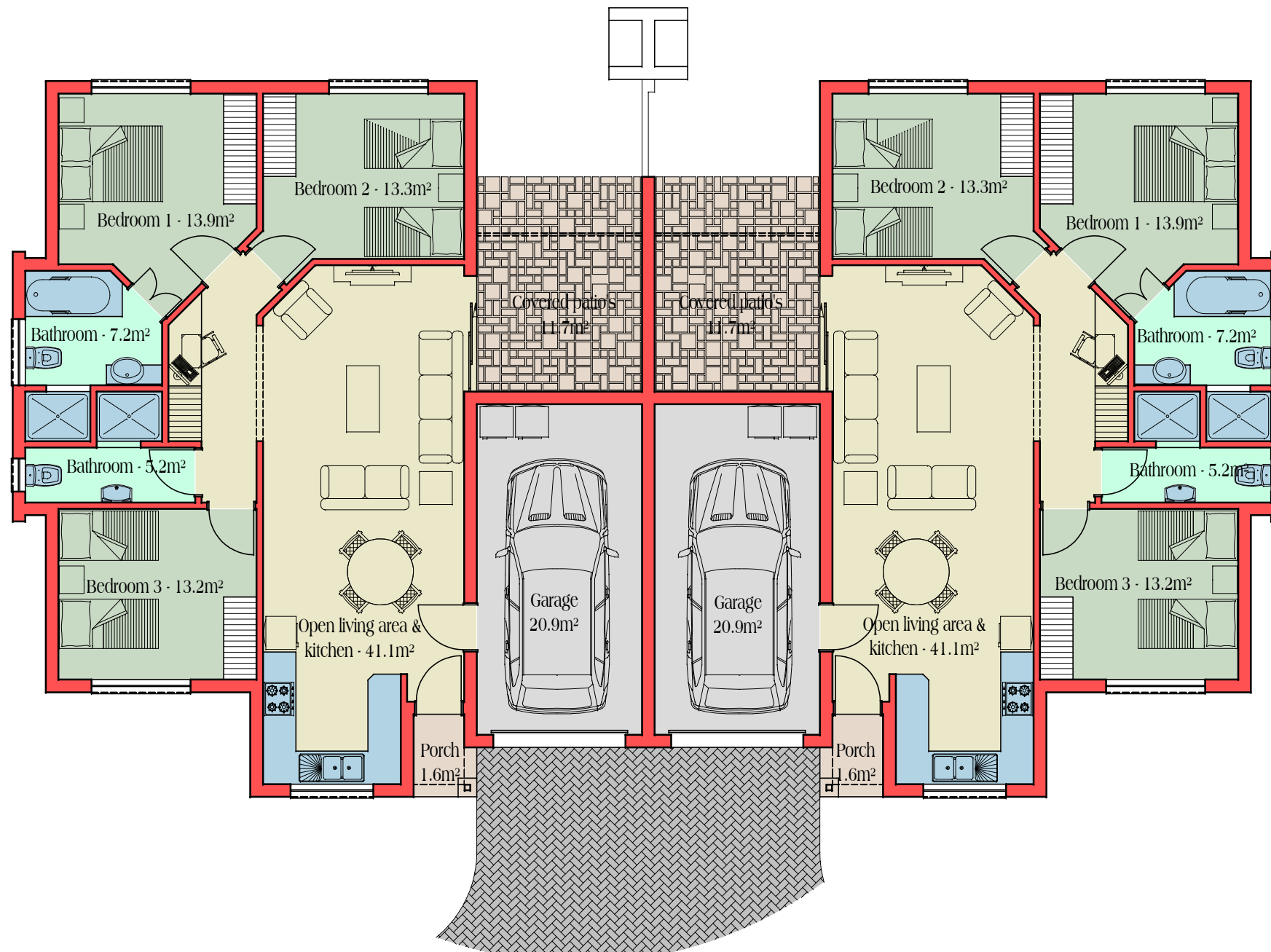
Floor plan
