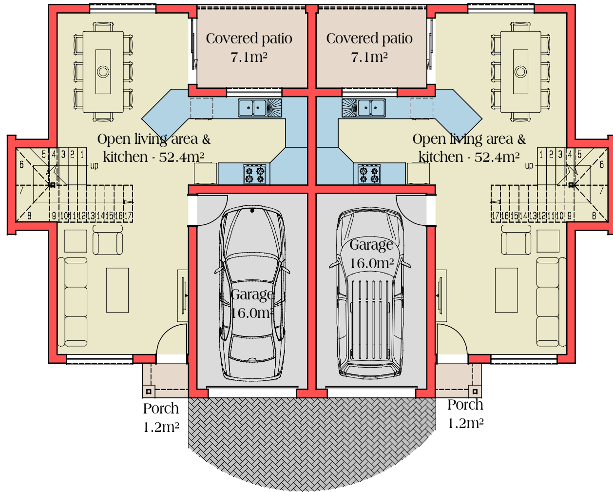
Ground floorplan
